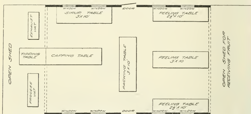
FIG. 6.—Floor plan of a small cannery.
